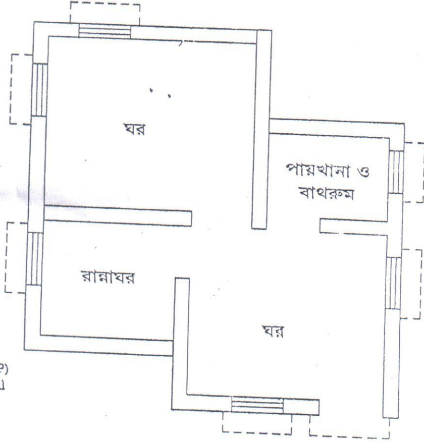
Gr. Floor Plan
